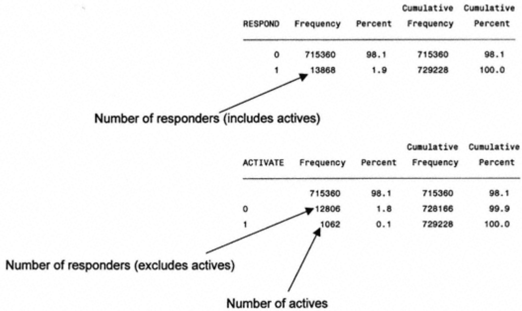
Figure 3.3 Sample frequencies.
